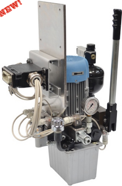
Rotor Brake - Wind Mill
